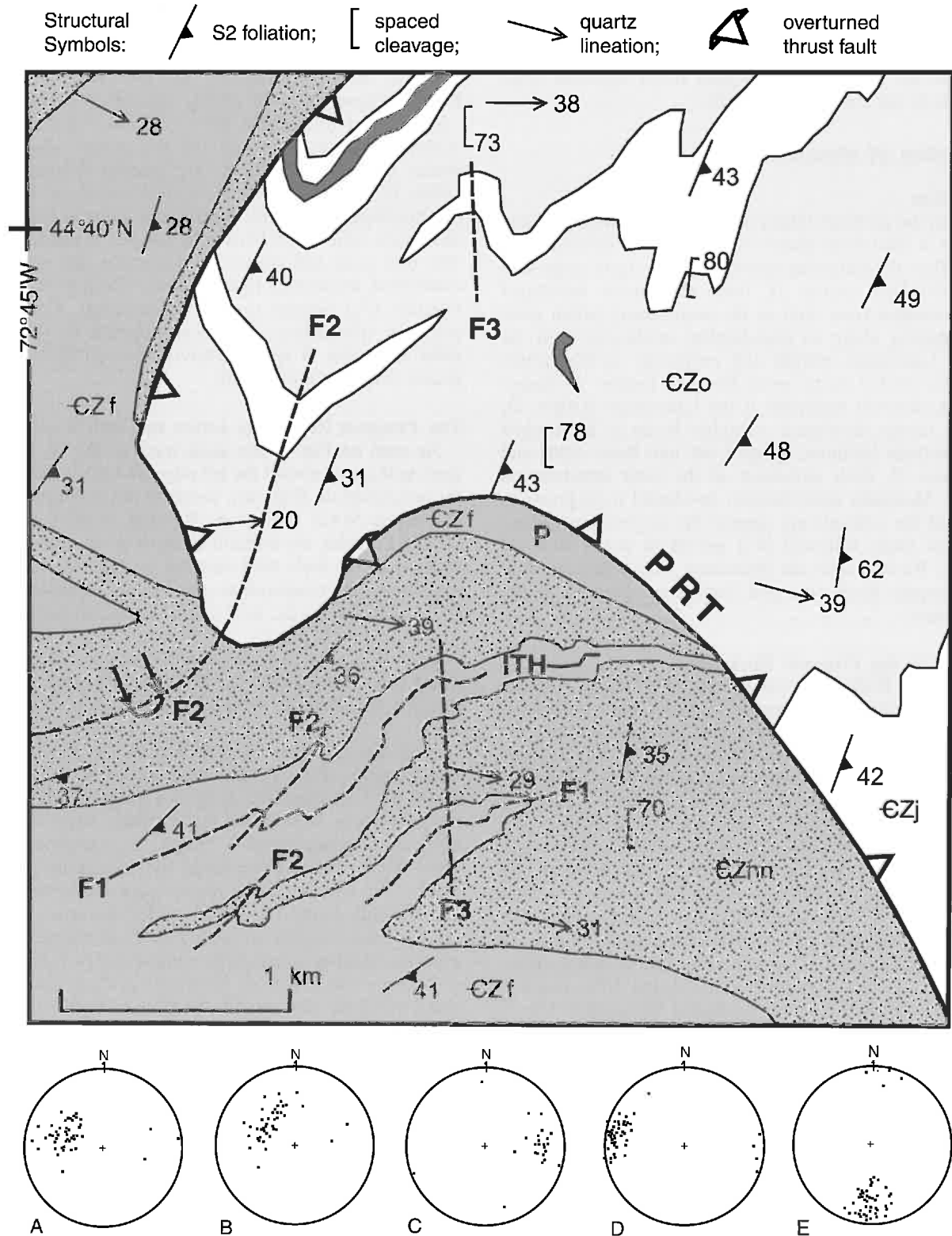
Fig. 6. Geologic map of the Prospect Rock area on the east limb of the Green Mountain anticlinorium. Rock units and abbreviations as in Fig. 4. ITH, Ithiel Falls. Structural Symbols: Dashed line, representative axial traces of folds. Equal area nets show structural data from area of Fig. 6. (A) Poles to S_2 (pervasive foliation) from upper plate of Prospect Rock thrust. (B) Poles to S_2 from lower plate of Prospect Rock thrust. (C) Quartz lineations from both plates. (D) Poles to S_3 (Acadian spaced cleavage). (E) F_3 fold axes.
