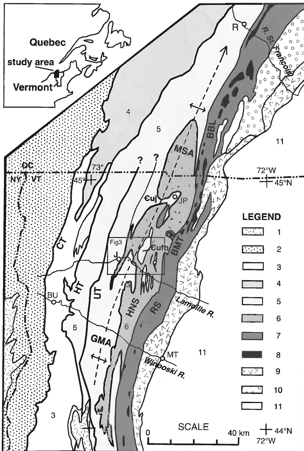
Fig. 1. Lithotectonic packages in northwestern Vermont and adjacent Quebec, after Stanley and Ratcliffe (1985), Slivitsky and St. Julien (1987), and Doll et al. (1961). Faults labeled on upper plate. Lithotectonic packages (legend boxes arranged from west to east): 1, Grenville basement; 2, Cambrian–Ordovician shelf; 3, Champlain slice; 4, Quebec allochthons; 5, Hinesburg (Oak Hill Group) and Underhill slices; 6, Hazens Notch slice; 7, Rowe slice; 8, ultramafics; 9, Moretown–Ascot arc-related rocks; 10, Late Ordovician flysch; 11, Silurian–Devonian rocks. BBL, Baie Verte–Brompton line; BMT, Belvidere Mountain thrust; BU, Burlington; CT, Champlain thrust; \epsilon_{ufb} , Underhill Formation, Foot Brook Member; \epsilon_{uj} , Underhill Formation, Jay Peak Member; GMA, Green Mountain anticlinorium; HNS, Hazens Notch slice; HT, Hinesburg thrust; J, Jeffersonville; JP, Jay Peak; MSA, Monts Sutton anticlinorium; MT, Montpelier; R, Richmond; RS, Rowe slice; UT, Underhill thrust.
