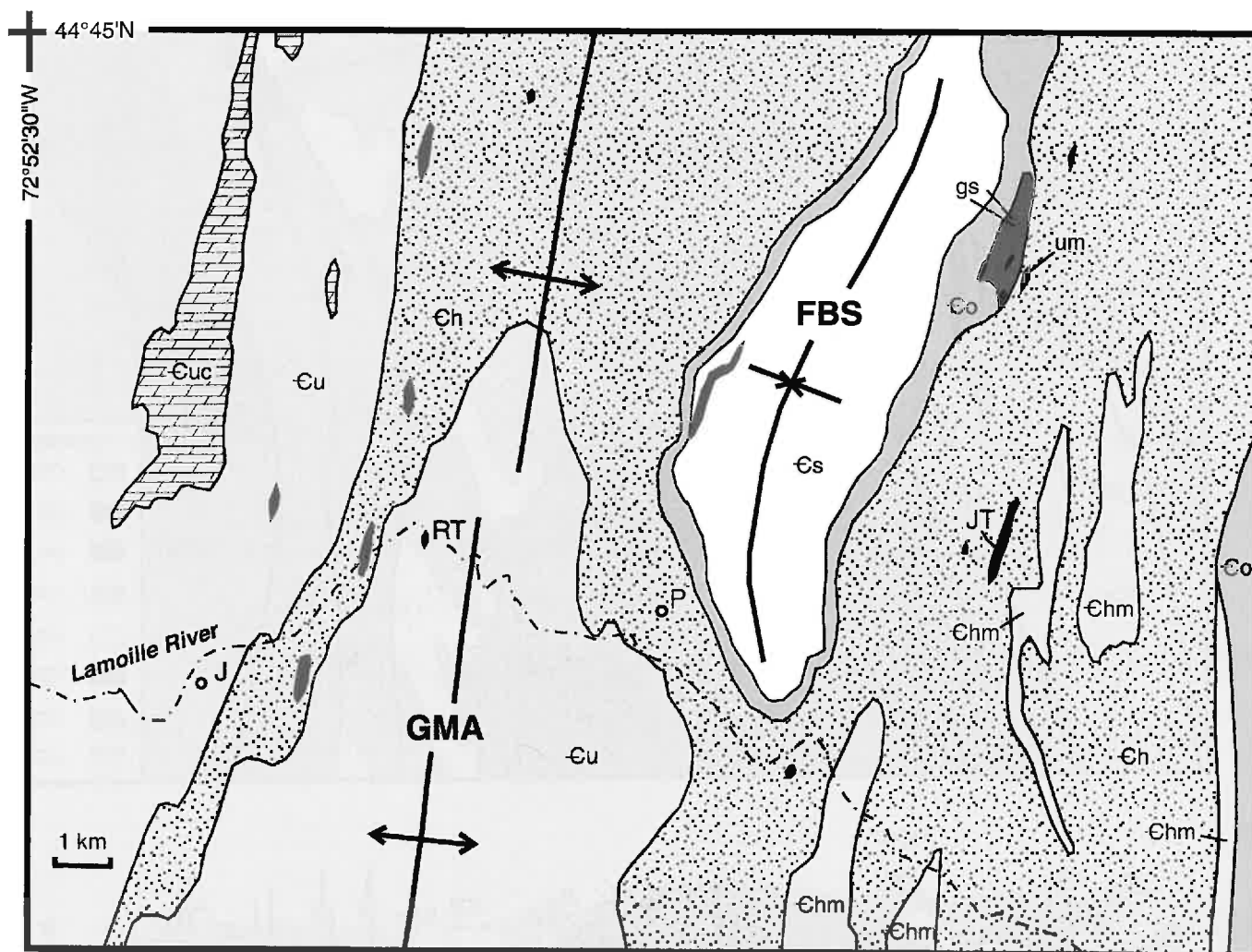
Fig. 3. Geologic map across the Green Mountain anticlinorium at the latitude of the Lamoille River, after Doll et al. (1961), Christman (1959), and Albee (1957). Rock units: -Eu, Underhill Formation.; -Euc, Underhill Formation carbonaceous member with dolostones; -Ch, Hazens Notch Formation; -Chm, Hazens Notch Formation, magnetite schist member; -Co, Ottauquechee Formation; -Es, Stowe Formation; gs, greenstones; um, ultramafics. FBS, Foot Brook syncline; GMA, Green Mountain anticlinorium; J, Jeffersonville; JT, Johnson talc mine; P, Prospect Rock; RT, Rousseau talc mine.
