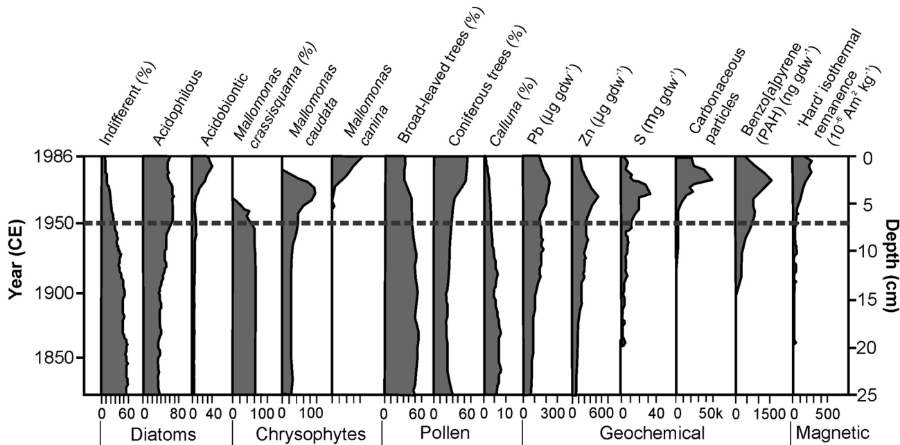
Fig. 18. Physical, chemical and biological trends from Lilla Öresjön (SW Sweden), a high-sulphate deposition area (from Renberg and Battarbee, 1990).
