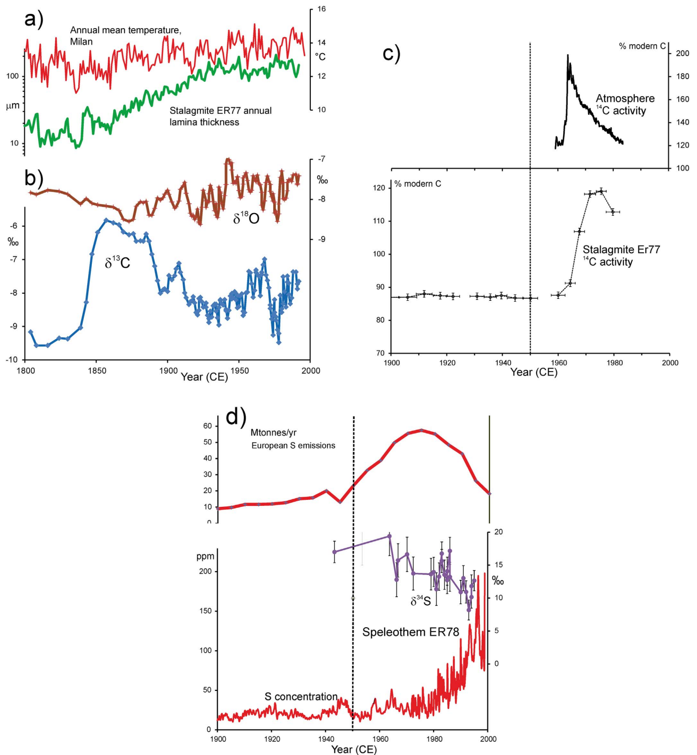
Fig. 29. Ernesto Cave, Italy: a) Age model based on lamina counting related to local mean air temperature (Frisia et al., 2003); b) \delta^{18}\text{O} and \delta^{13}\text{C} profiles (Scholz et al., 2012); c) Radiocarbon profile and comparable European atmospheric emissions (Fohlmeister et al., 2011); d) S concentration and \delta^{34}\text{S} (Frisia et al., 2005; Wynn et al., 2010).
