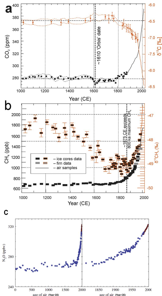
Fig. 27. a) Law Dome ice core and firn records for CO 2 concentration and δ 13 C for atmospheric CO 2 for the past 1000 years (from Rubino et al., 2013); b) Law Dome ice core and firn records for CH 4 concentration and δ 13 C for atmospheric CH 4 for the past 1000 years (from Ferretti et al., 2005); c) N 2 O concentrations in the Law Dome ice core over the past 2000 years and 200 years (Wolff, 2013).
