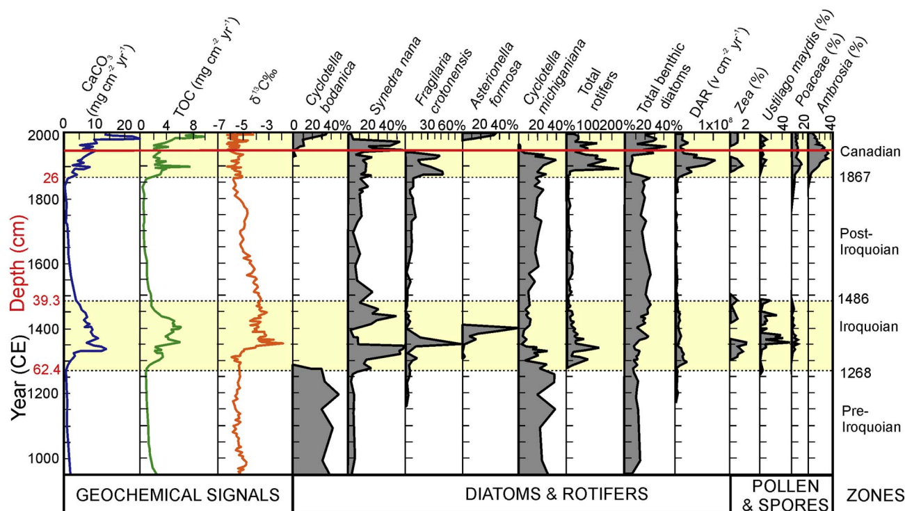
Fig. 16. Stratigraphic signals of the last millennium in Crawford Lake, Canada. The horizontal red line near the top is the ~1950 CE level, marked by both lithological and biostratigraphic changes in available data. From Zalasiewicz et al. (2017a), modified after Ekdahl et al. (2004). DAR is diatom accumulation rate.
