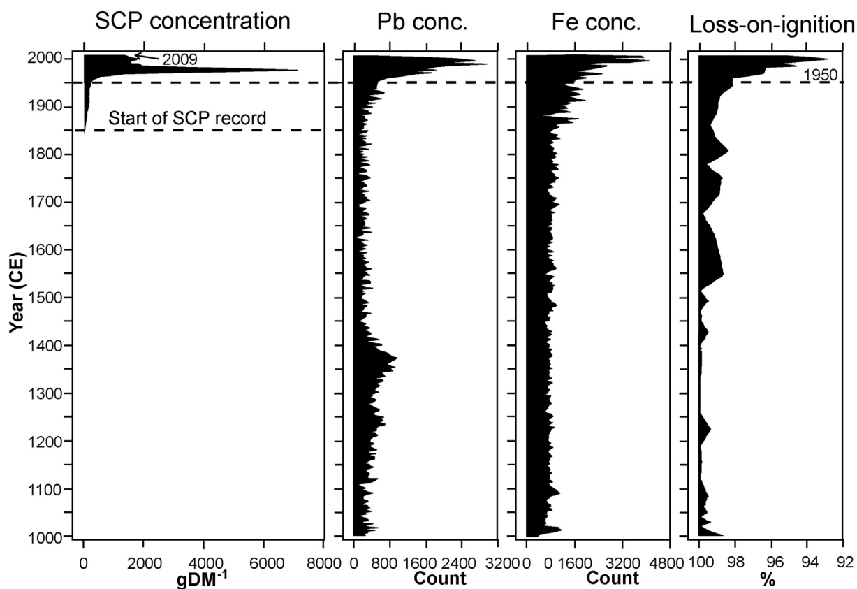
Fig. 22. Spheroidal carbonaceous particles (SCPs), lead and iron concentrations from Malham Tarn Moss, England (from Swindles et al., 2015).
