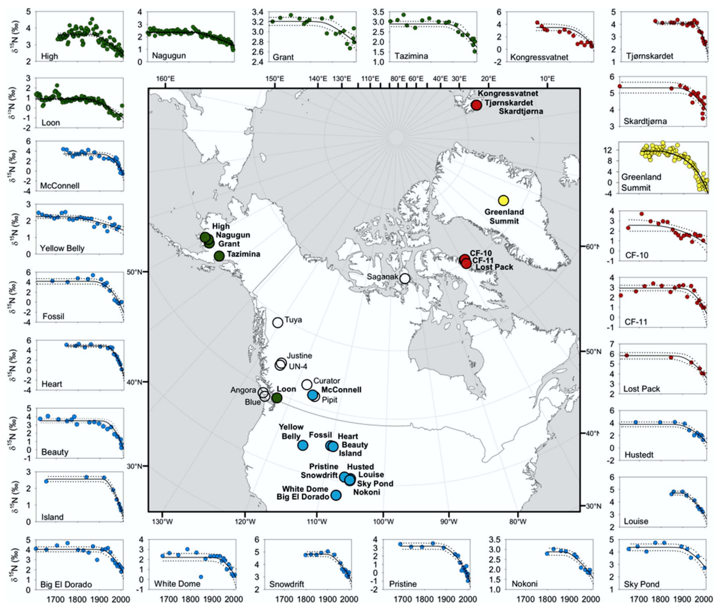
Fig. 14. Sediment \delta^{15}\text{N} profiles from Northern Hemisphere lakes (from Holtgrieve et al., 2011). Lake ecotypes include: temperate/boreal (green circles), alpine (blue circles), and arctic (red circles), and the Greenland Summit ice core is indicated with a yellow circle. The solid lines are the median posterior fits to the observed data using the most parsimonious model, and the dotted lines are the 2.5 and 97.5% credible limits.
