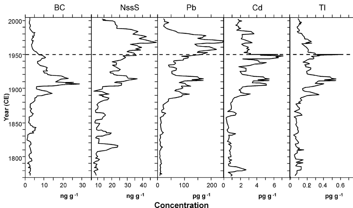
Fig. 26. Concentrations (5-year running means) in Greenland ACT2 ice core from 1772 to 2003 CE of sulphur (NssS), thallium (Tl), cadmium (Cd) and lead (Pb), compared to black carbon (BC), from McConnell and Edwards (2008). Sulphur peaks in 1817 and 1883 CE relate to the Tambora and Krakatoa volcanic eruptions, respectively. © (2008) National Academy of Sciences, U.S.A.
