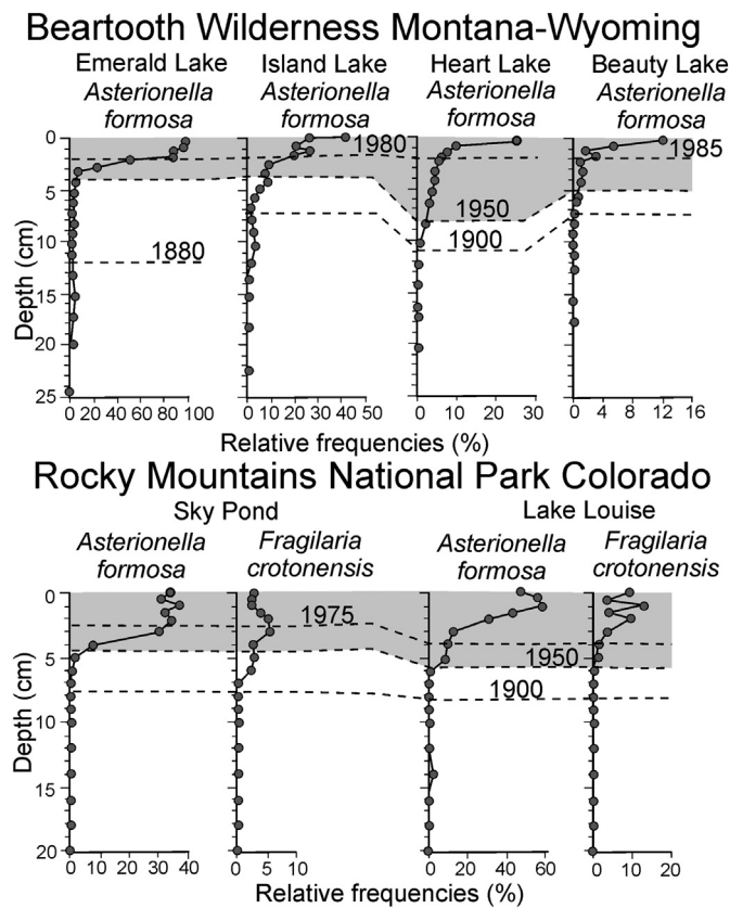
Fig. 15. Replacement of Holocene diatom assemblages by Asterionella formosa and/or Fragilaria crotonensis mainly in lake cores from US high-altitude sites, since ~1950 CE (Saros et al., 2005). Location of lakes shown on Fig. 14.
