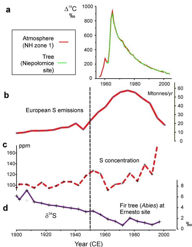
Fig. 32. a) Tree rings ( Pinus sylvestris ) samples from 1960 to 2003 CE at Niepołomice (Poland) showing changes of radiocarbon concentration (from Rakowski et al., 2013) compared with Northern Hemisphere (Zone 1) atmospheric values (from Hua and Barbetti, 2004); b) European S emissions; c) S concentrations; and d) \delta^{34}\text{S} in Abies alba from NE Italy compared with European S emissions (Wynn et al., 2014).
