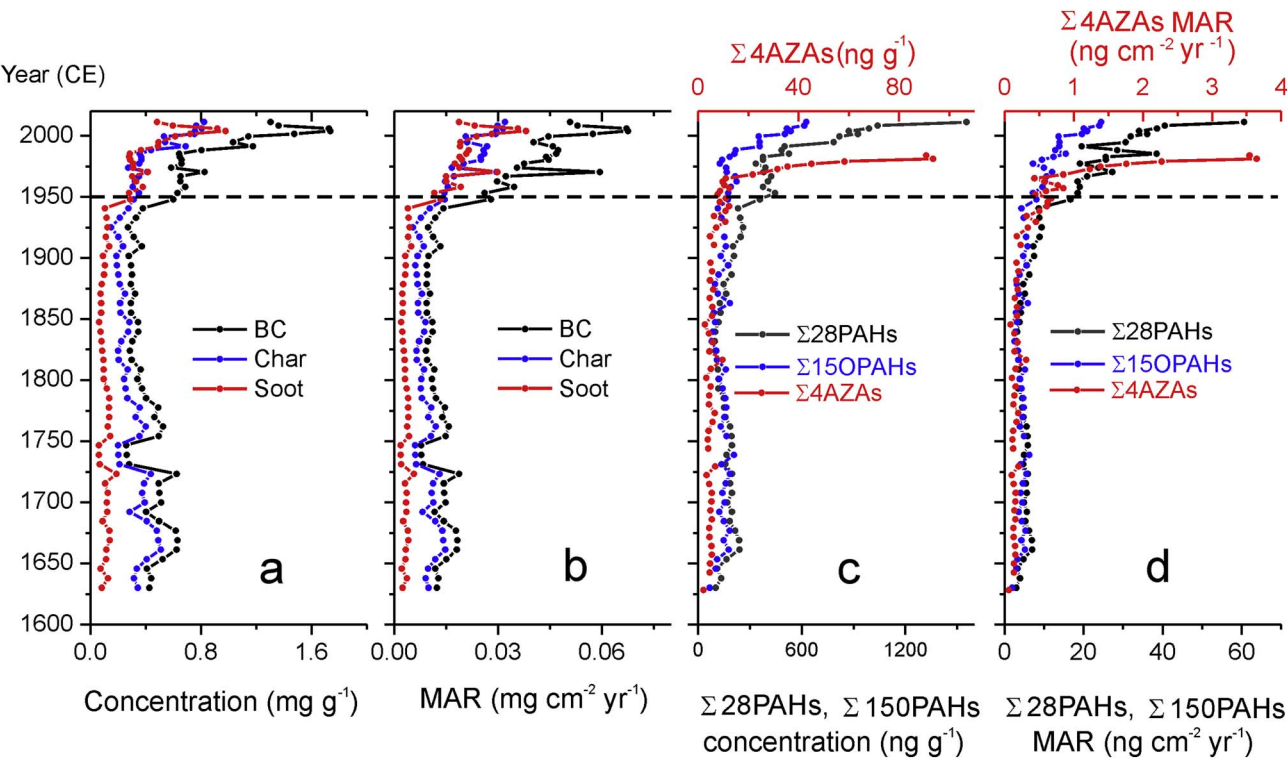
Fig. 19. Historical variations of concentrations and mass accumulation rates (MARs) of black carbon (BC), char, and soot, parent-PAHs, oxygenated PAHs (OPAHs), and azaarenes (AZAs) in the Huguangyan Maar Lake (from Han et al., 2016).
