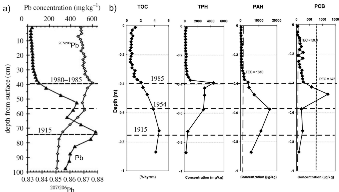
Fig. 9. Example of data from a single core from the Clyde Estuary showing a) Pb concentrations and 207/206 Pb isotope ratios, and b) PAH, TPH and PCB organic chemical signatures (Vane et al., 2011). Dates are interpreted.
