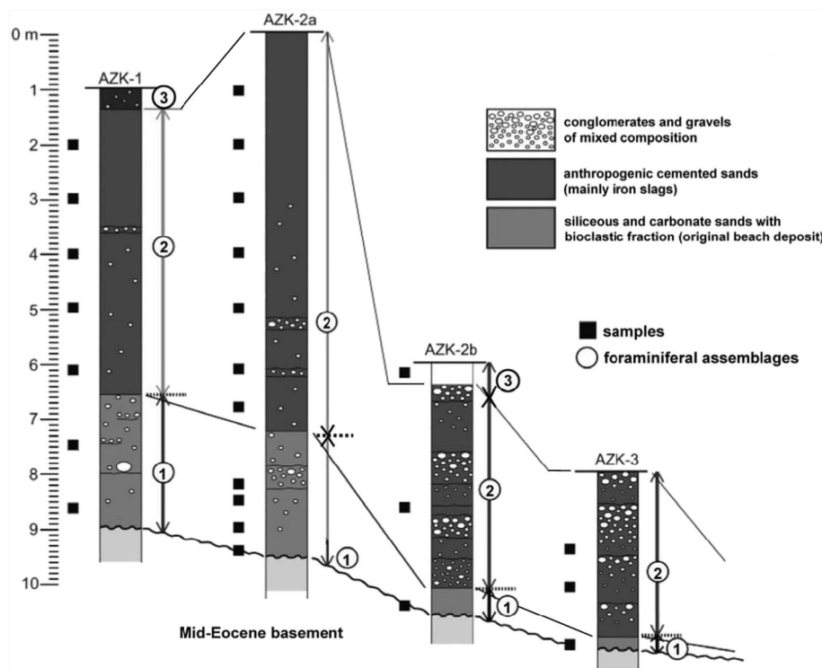
Fig. 2. Cores through the Gorrondatxe-Tunelboca beachrock, Spain. A natural high-energy open beach sand deposit, pre-dating the discharges of iron slag, is overlain by cemented sandy and coarse beach deposits that are commonly conglomeratic with abundant slag clasts and incorporating littoral foraminifera. Three distinct foraminiferal assemblages are recognised (ranges for assemblages 1, 2 and 3 marked by arrows). Modified from Martínez-García et al., 2013.
