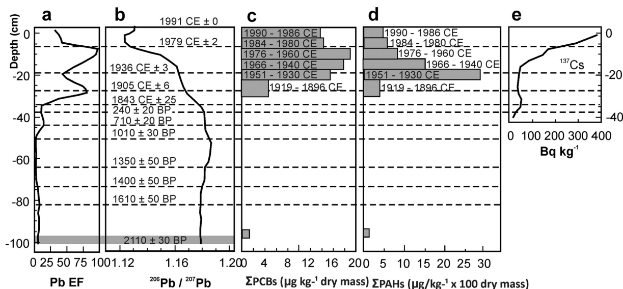
Fig. 21. Core from Etang de la Gruère, Switzerland, collected in 1991 CE: a) Pb Enrichment Factor (EF) calculated as the ratio of Pb/Sc in the peats, normalized to the background value (from Shotyk et al., 1998); b) Pb isotopic values (from Shotyk et al., 1998); c) ΣPCBs (from Berset et al., 2001); d) ΣPAHs (from Berset et al., 2001); e) ^{137}\text{Cs} (from Appleby et al., 1997). Succession dated using ^{210}\text{Pb} to 35 cm depth (Appleby et al., 1997) and ^{14}\text{C} yr BP from 35 cm to base (Shotyk et al., 1998).
