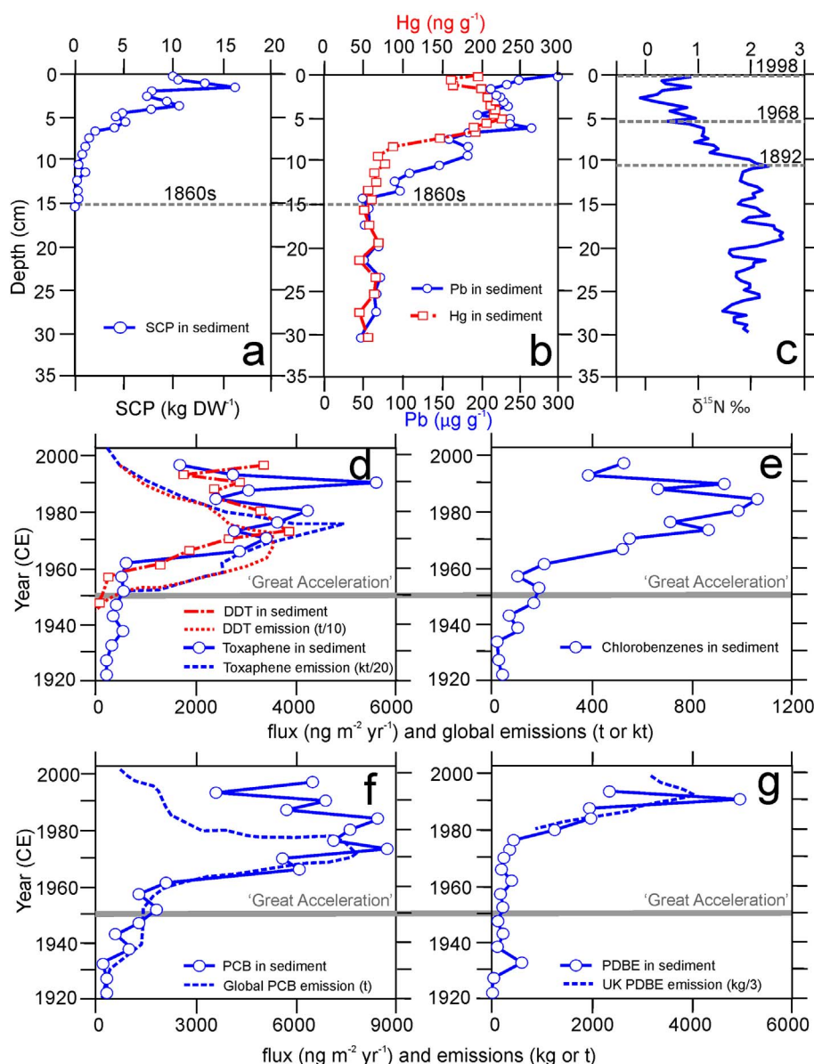
Fig. 17. Contamination record in Lochnagar sediments (Scotland) demonstrating appearances as post-mid-20th century markers: (a) spheroidal carbonaceous particles (SCPs) (from Yang et al., 2002a); (b) Hg and Pb (from Yang et al., 2002a); (c) \delta^{15}\text{N} (from Curtis and Simpson, 2011); (d) the chlorinated pesticides DDT and toxaphene from core collected in 1997 CE related to emission data (from Muir and Rose, 2007); (e) chlorobenzenes (from Muir and Rose, 2007); (f) total PCBs related to global emissions (from Muir and Rose, 2007); and (g) PDBEs related to UK emissions (from Muir and Rose, 2007).
