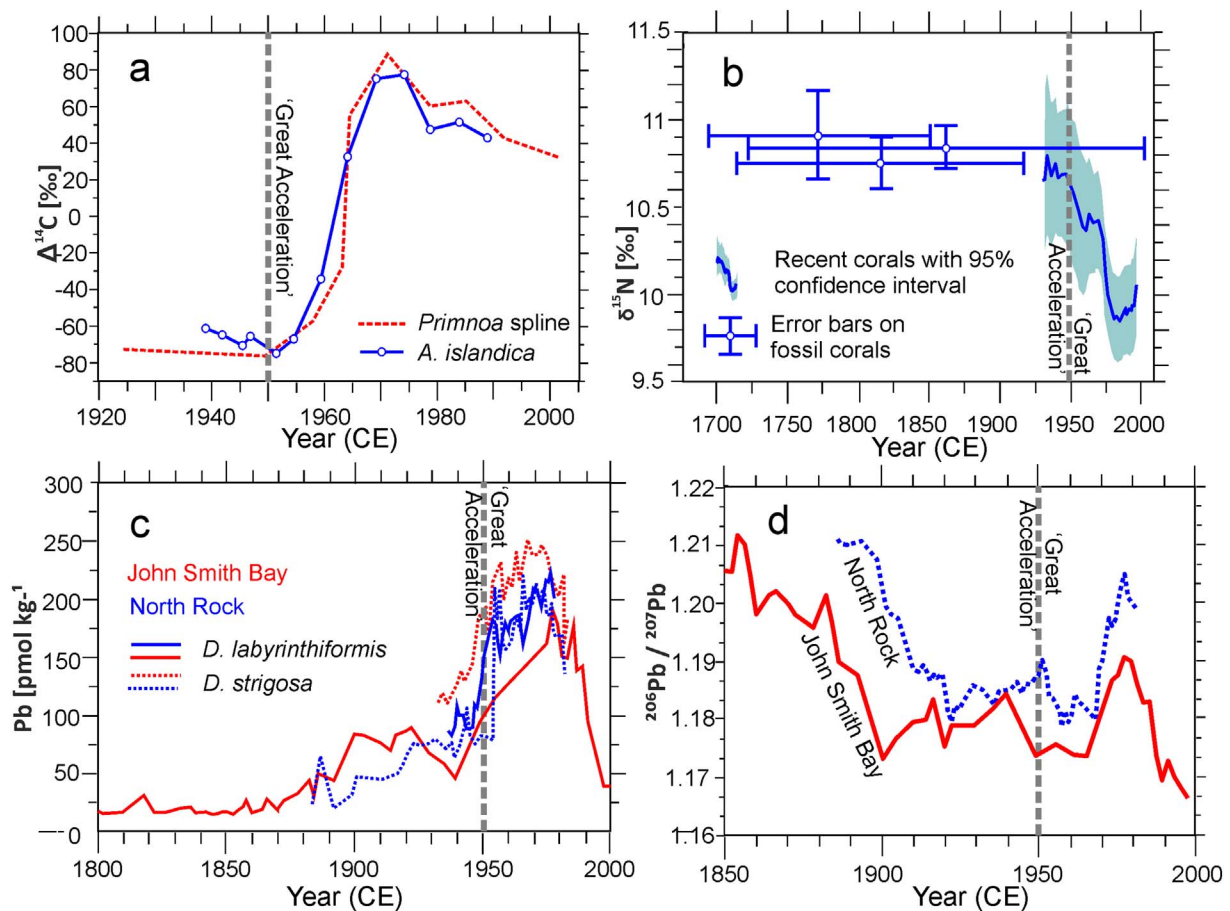
Fig. 7. a) Plot of \Delta^{14}\text{C} vs age for 7 different colonies of the deep-sea gorgonian coral Primnoa resedaeformis with spline fit through the data (Sherwood et al., 2005a), and for the bivalve Arctica islandica (Weidman and Jones, 1993); b) decreased \delta^{15}\text{N-AA} values in deep-sea gorgonian corals in the NW Atlantic (Sherwood et al., 2011) © (2011) National Academy of Sciences; c) Pb concentration; and d) ^{206}\text{Pb}/^{207}\text{Pb} in Bermuda corals (Kelly et al., 2009).
