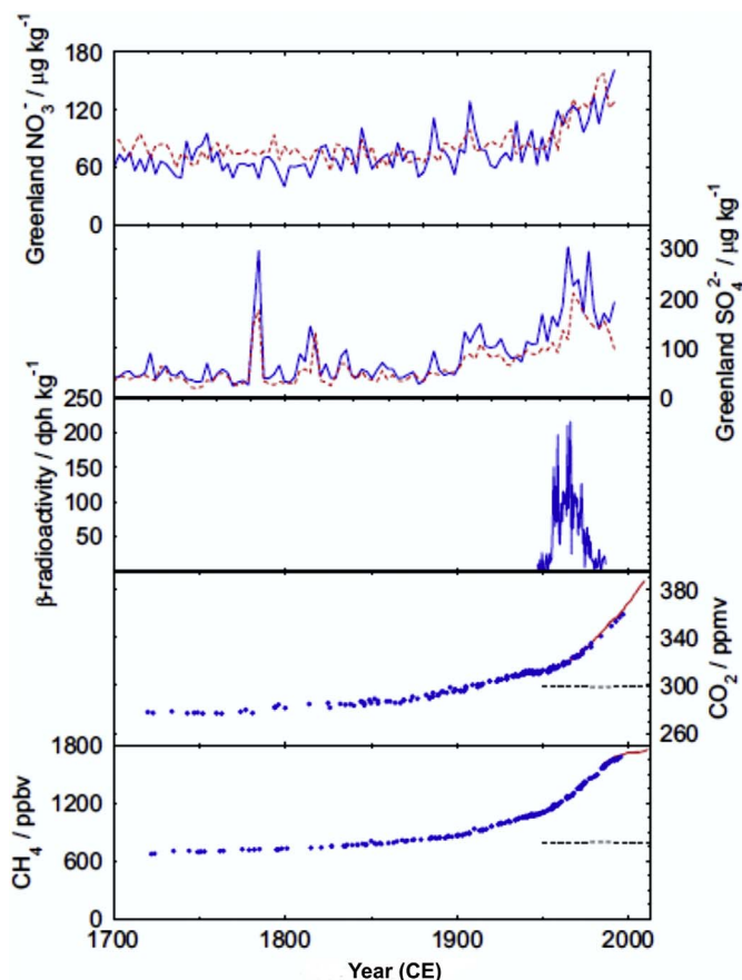
Fig. 25. Ice core signals since 1700 CE (from Wolff, 2014). \text{CH}_4 and \text{CO}_2 ice-core data (blue dots) are from Law Dome, Antarctica (MacFarling Meure et al., 2006), and recent atmospheric data (red lines) from Mauna Loa ( \text{CO}_2 ) and Cape Grim ( \text{CH}_4 ) observatories. The horizontal dashed lines are the highest values observed in ice cores of the last 800,000 years prior to the period shown. Beta radioactivity is from Coats Land, Antarctica (Wolff et al., 1999). Sulphate and nitrate are shown for two cores from Greenland: B16 (dashed red) and B21 (solid blue) (Fischer et al., 1998). The 18th- and 19th-century spikes in sulphate are signals of volcanic eruptions.
