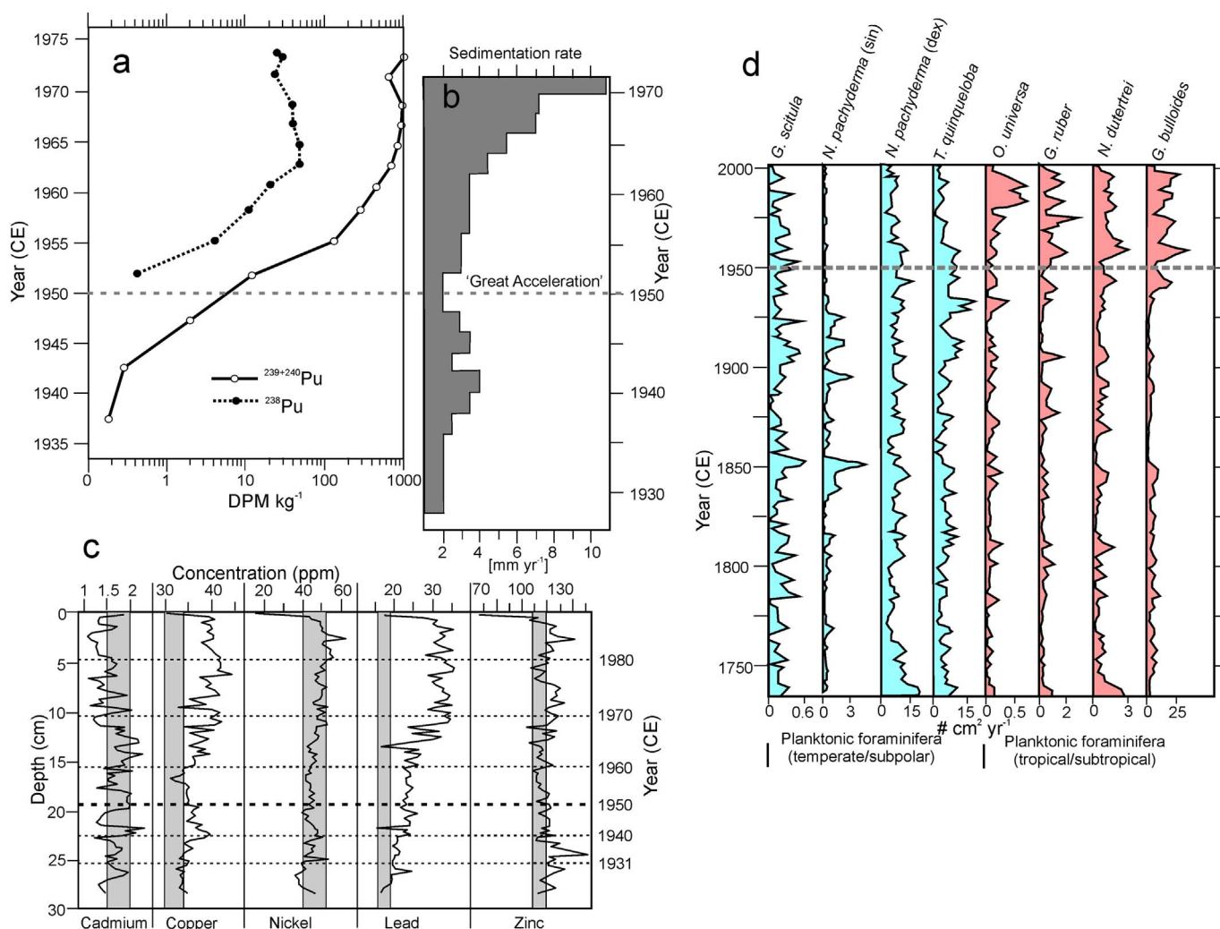
Fig. 4. Key signals in marine cores from the Santa Barbara Basin, with a) Pu signal (Koide et al., 1975), b) variations in sedimentation rates (Krishnaswami et al., 1973), c) selected heavy metals (Schmidt and Reimers, 1991) and d) planktonic foraminifera (Field et al., 2006).
