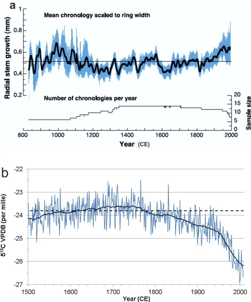
Fig. 31. a) The 20-year smoothed Northern Hemisphere extra-tropics reconstruction of radial stem productivity in high elevation and high latitude forest environments since 800 CE (black) and two-tailed 95% bootstrap confidence intervals (blue) (from Esper et al., 2002); b) δ 13 C variability from Loader et al. (2013a) for the period 1500–2008 CE measured in tree-ring cellulose for a composite tree ring stable isotope chronology developed using Pinus sylvestris trees from northern Fennoscandia. Fine line represents annually-resolved δ 13 C variability, thick solid line presents the annual data smoothed with a centrally-weighted 51-year moving average. Dashed line represents the mean δ 13 C value for the “pre-industrial” period 1500–1799 CE. Mean annual replication for the record is > 13 trees. Analytical precision σ n-1 = 0.12 per mille n = 951 which compares favourably with the analytical precision of the method typically reported (σ n-1 = 0.10 n = 10) (Boettger et al., 2007; McCarroll and Loader, 2004; Loader et al., 2013a).
