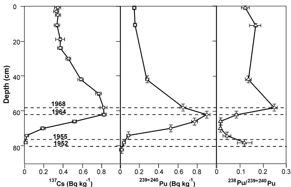
Fig. 13. Radiogenic signature from Lake Victoria, Australia (Hancock et al., 2011). Profiles of ^{137}\text{Cs} (closed squares), ^{239} + ^{240}\text{Pu} (open circles) and ^{238}\text{Pu}/^{239} + ^{240}\text{Pu} (triangles).
