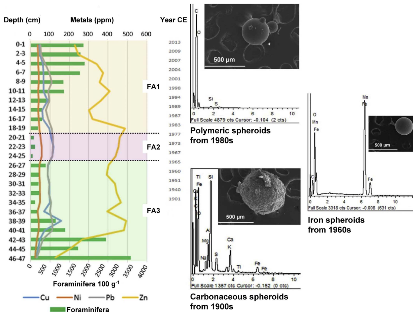
Fig. 10. Metal concentrations (Cu, Ni, Pb, Zn) versus foraminiferal density in the Urola estuary (northern Spain). FA1–FA3 represent three distinct foraminiferal assemblages referred to in the text. Modified from Goffard (2016).
